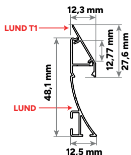
LUND T1 ALUMINIUM LED PROFILE / PROFIL LED 1 PC / 1 SZT.
