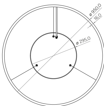
Ring FLEXA 950 mm | Widok z góry Ring FLEXA 950 mm | Top view
